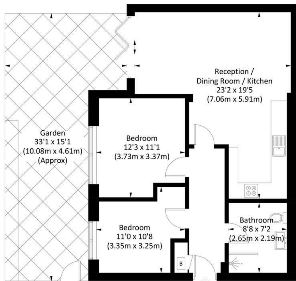
Ground Floor
